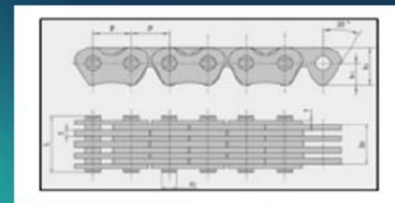
Toothed Timing Chain
